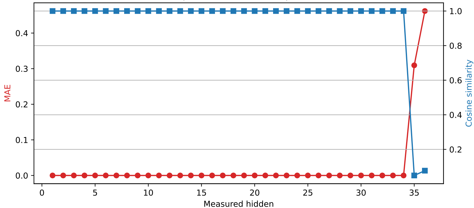
SmolLM3-3B | Quantized layer 34 | float32 \rightarrow int2
