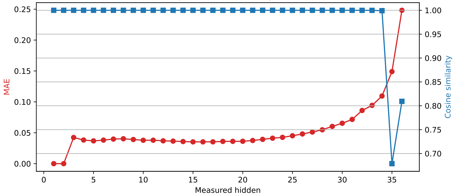
SmolLM3-3B | Quantized layer 2 | float64 → int2
