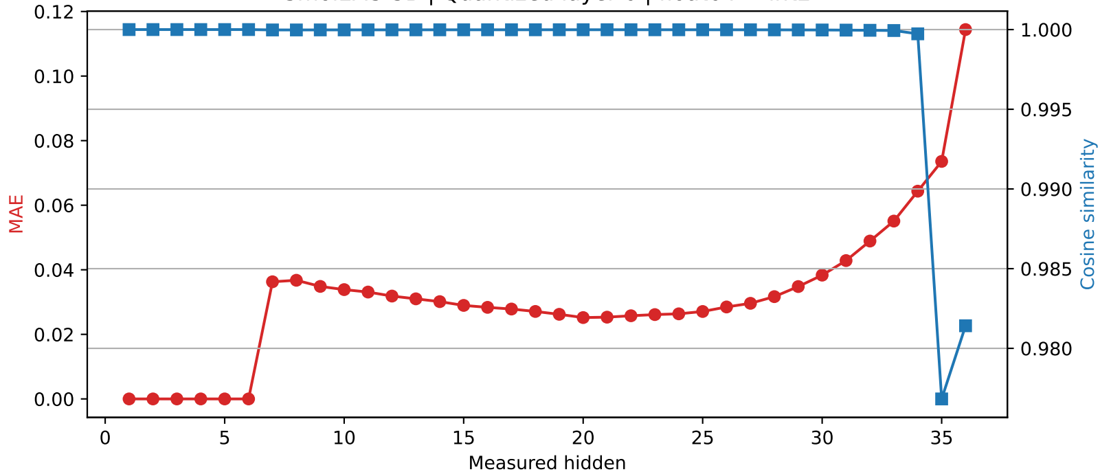
SmolLM3-3B | Quantized layer 6 | float64 → int2
