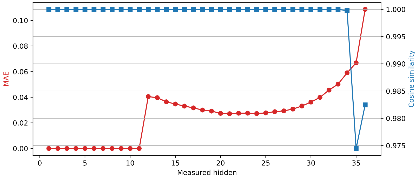
SmolLM3-3B | Quantized layer 11 | float64 → int2
