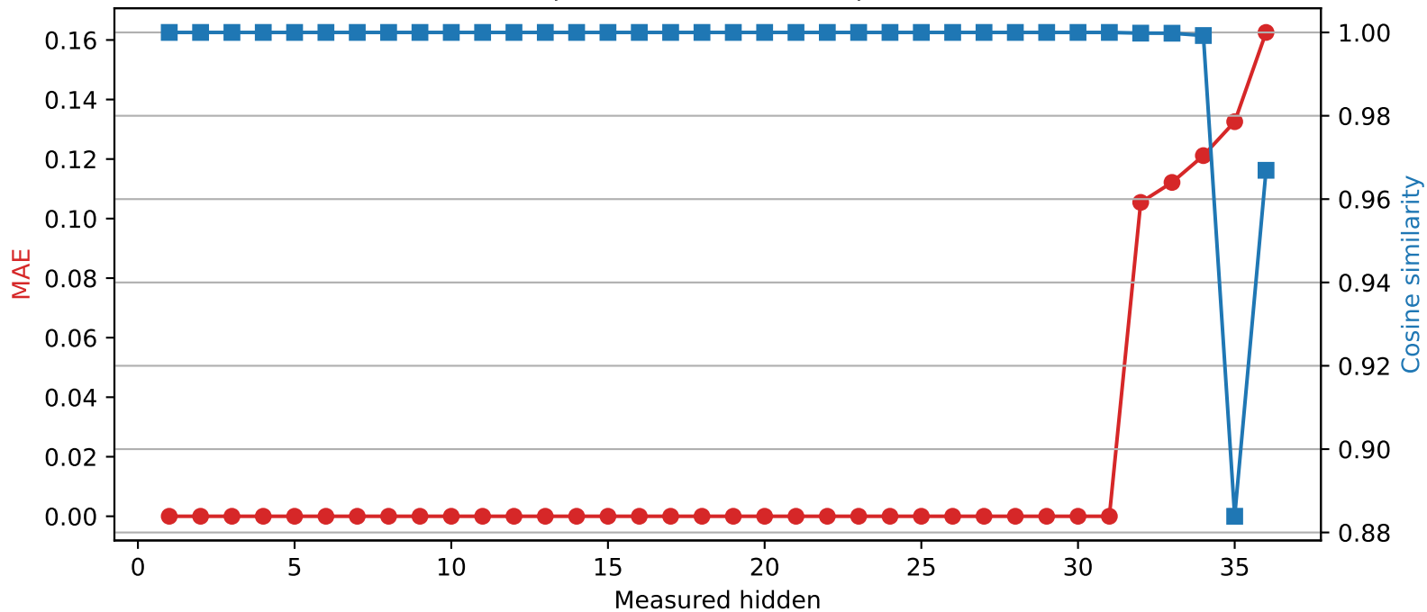
SmolLM3-3B | Quantized layer 31 | float64 → int2
