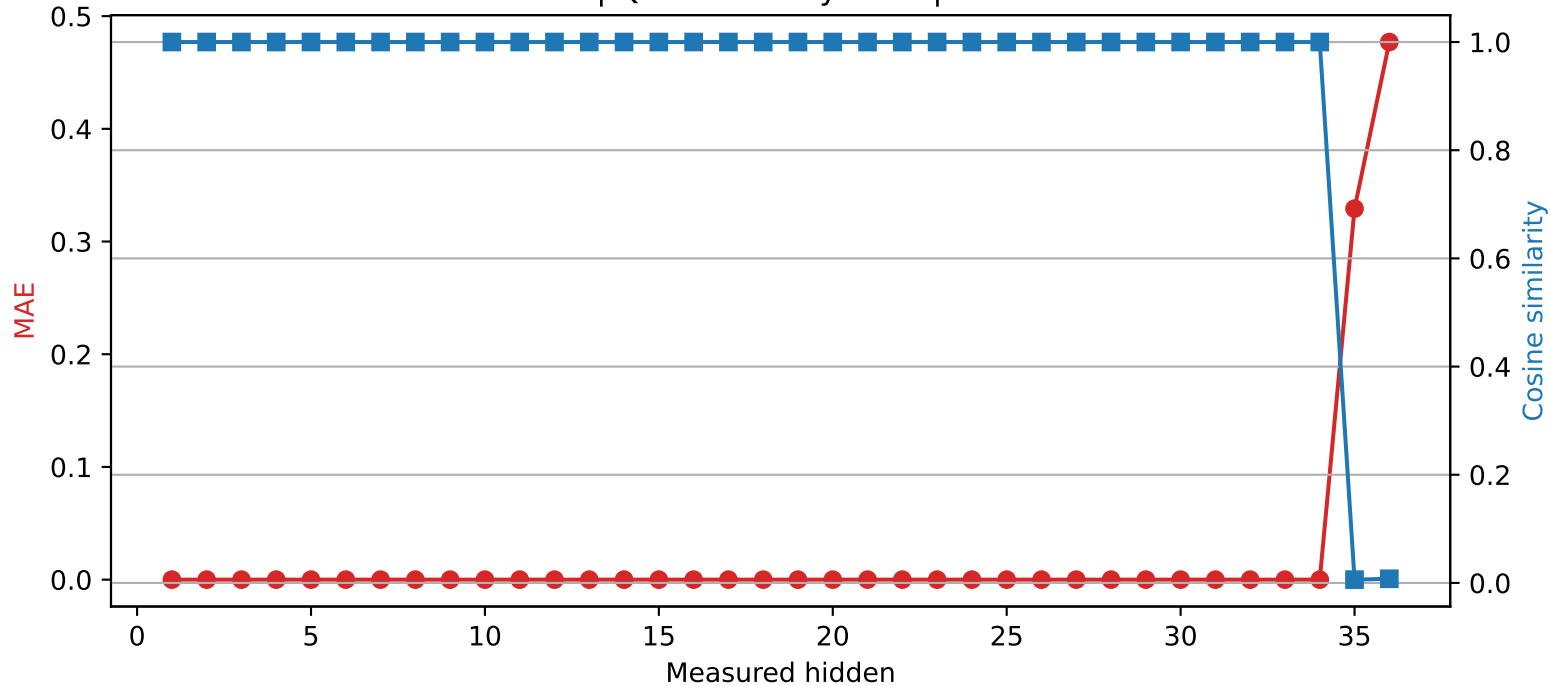
SmolLM3-3B | Quantized layer 34 | float64 → int2
