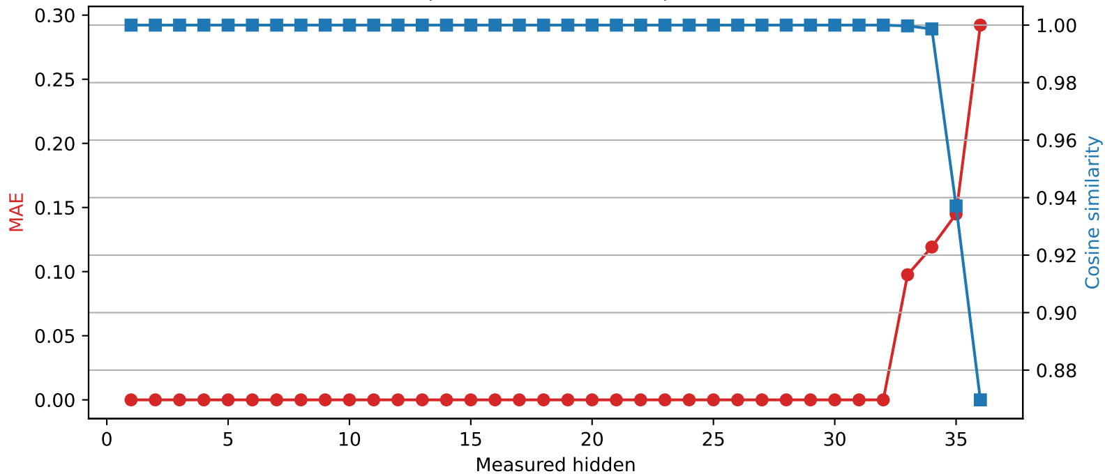
SmolLM3-3B | Quantized layer 32 | float64 → int2
