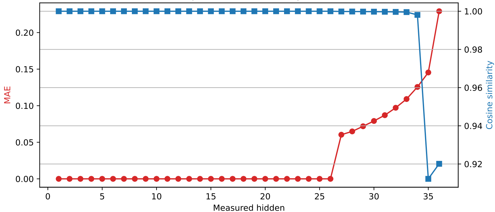
SmolLM3-3B | Quantized layer 26 | float64 → int2
