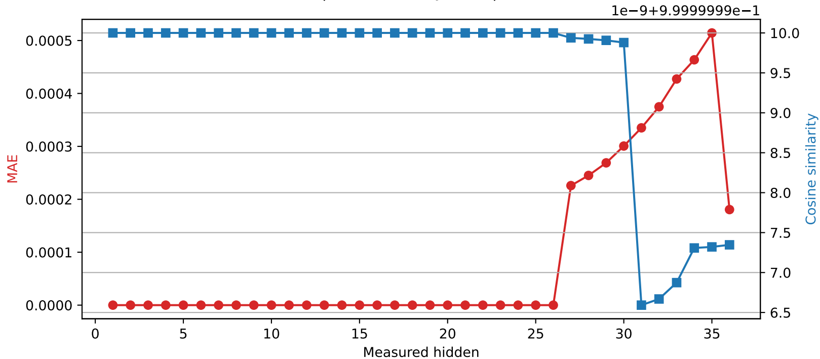
Qwen2.5-3B | Quantized layer 26 | float32 → int16
