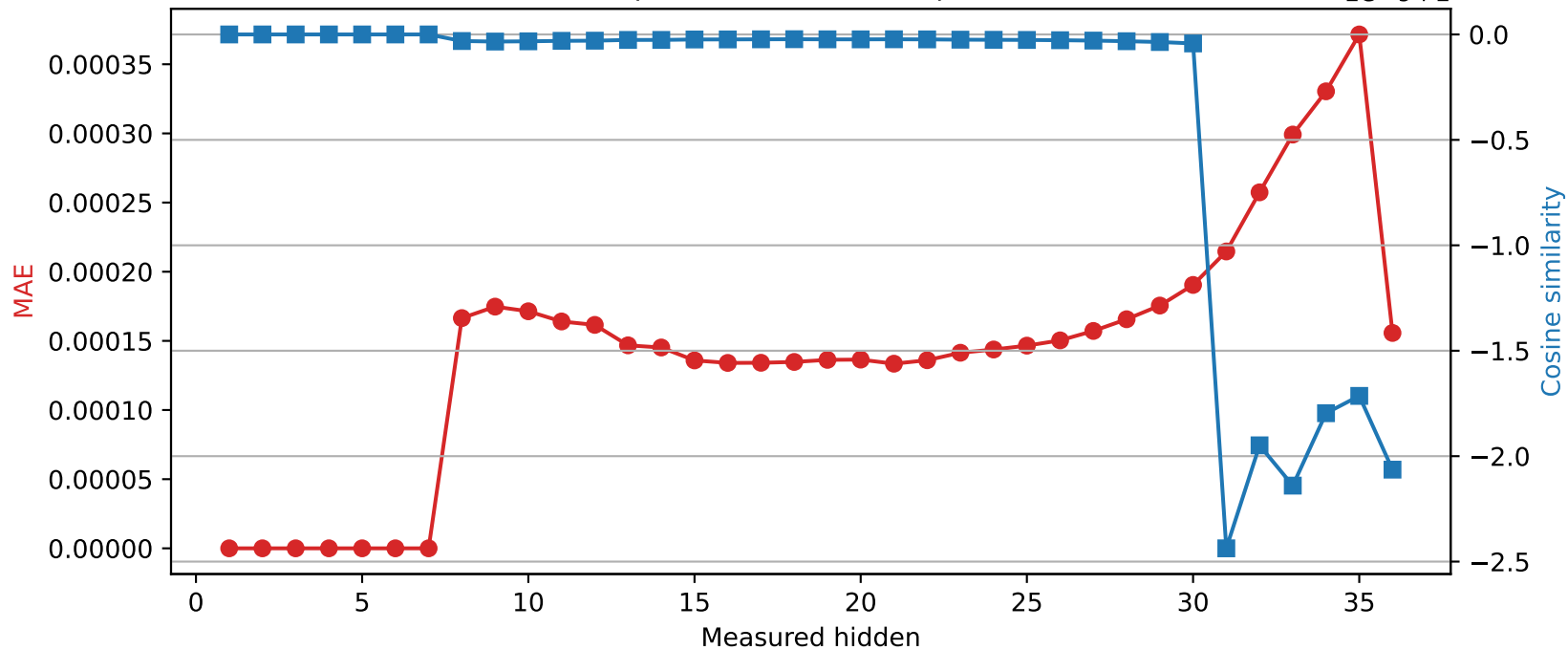
Qwen2.5-3B | Quantized layer 7 | float32 \rightarrow int16
