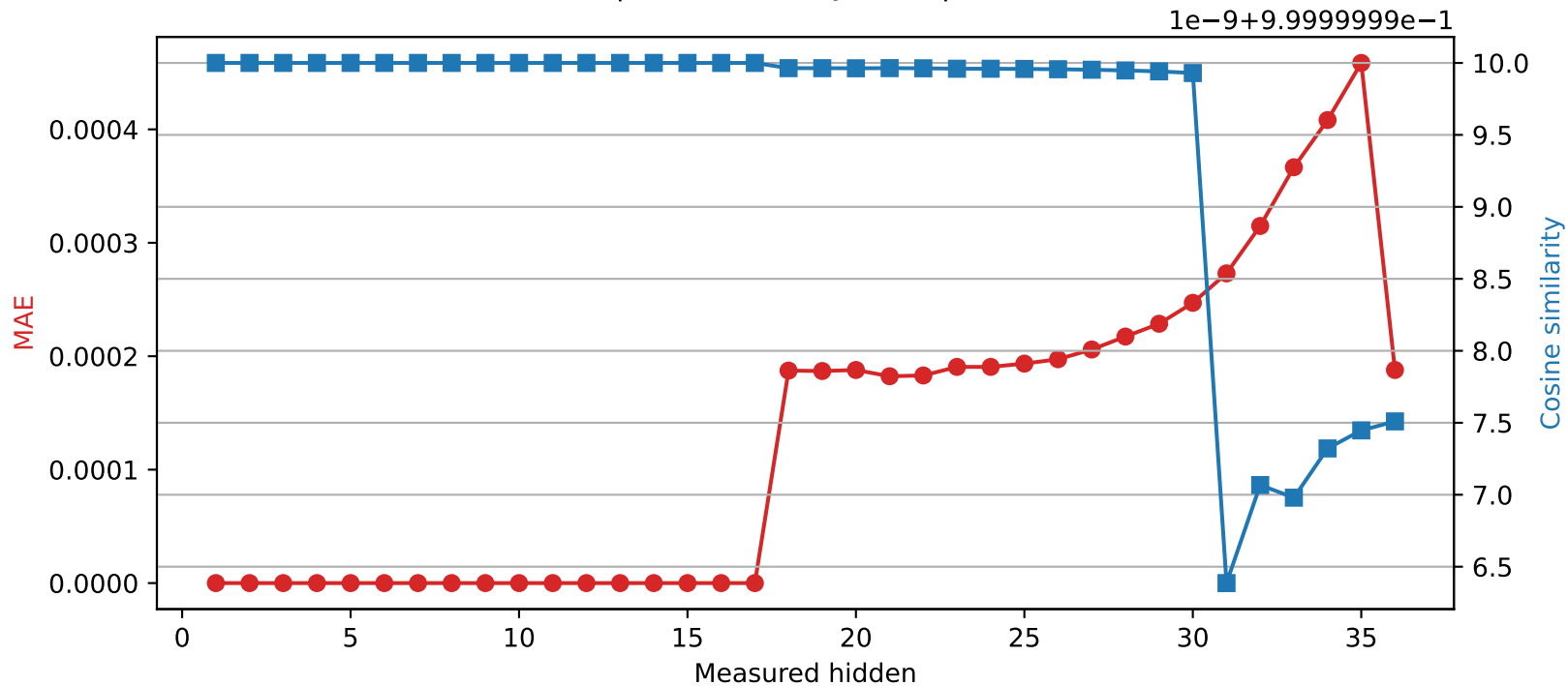
Qwen2.5-3B | Quantized layer 17 | float32 → int16
