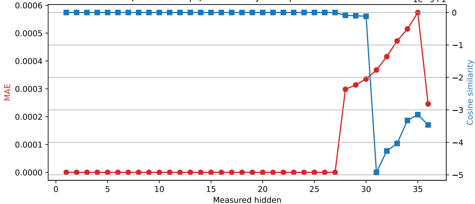
Qwen2.5-3B | Quantized layer 27 | float32 → int16
