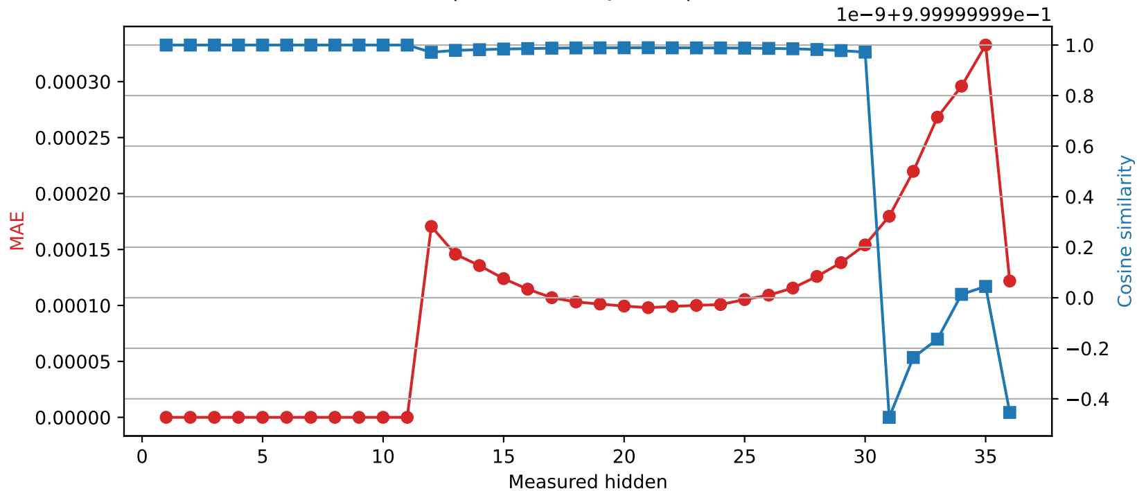
Qwen2.5-3B | Quantized layer 11 | float32 → int16
