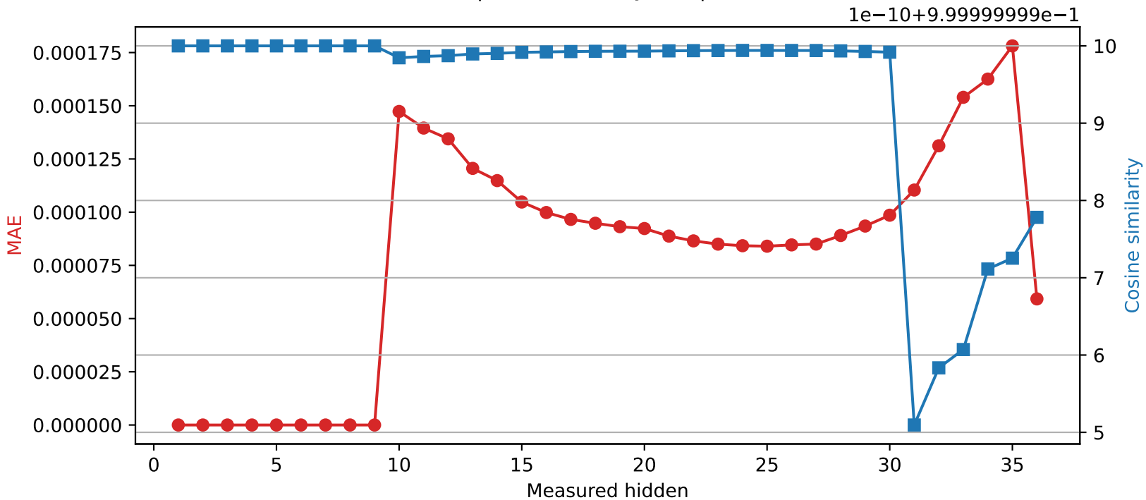
Qwen2.5-3B | Quantized layer 9 | float32 → int16
