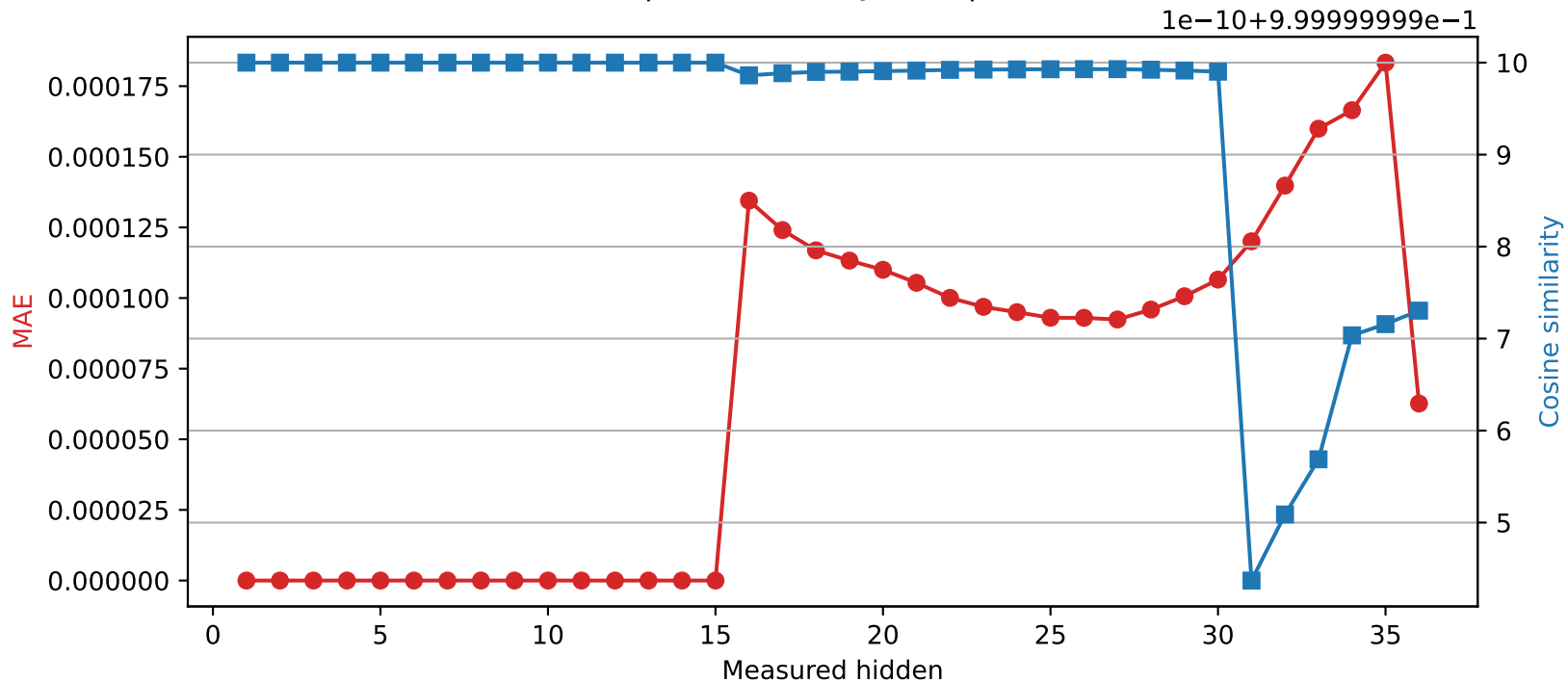
Qwen2.5-3B | Quantized layer 15 | float32 → int16
