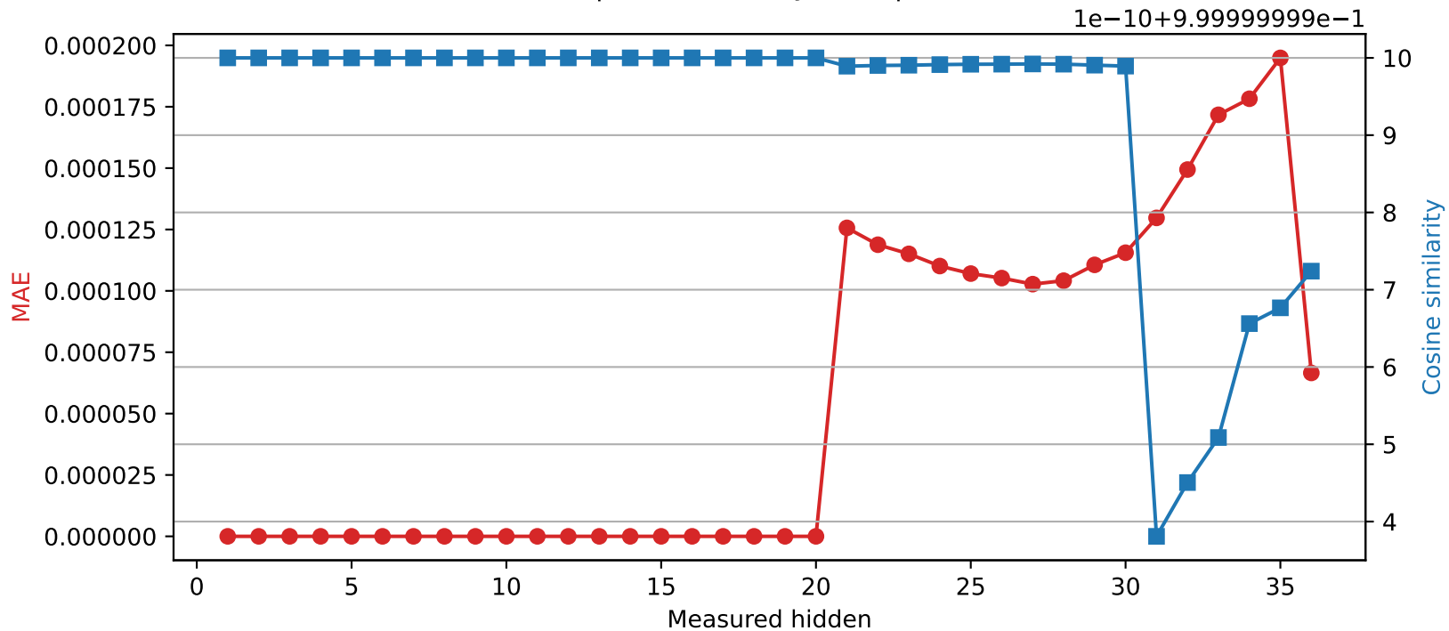
Qwen2.5-3B | Quantized layer 20 | float32 → int16
