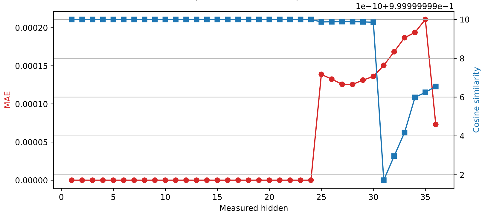
Qwen2.5-3B | Quantized layer 24 | float32 → int16
