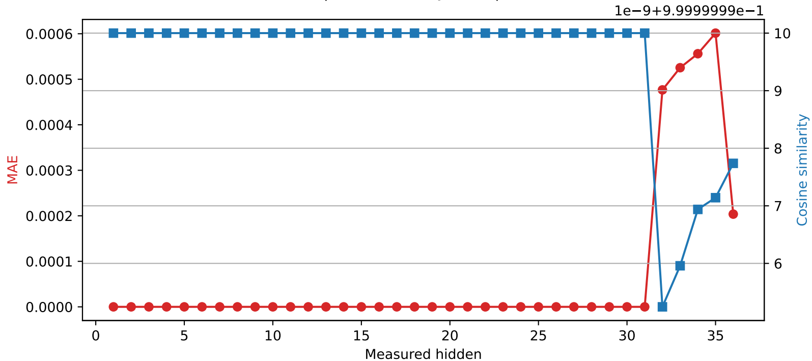
Qwen2.5-3B | Quantized layer 31 | float32 → int16
