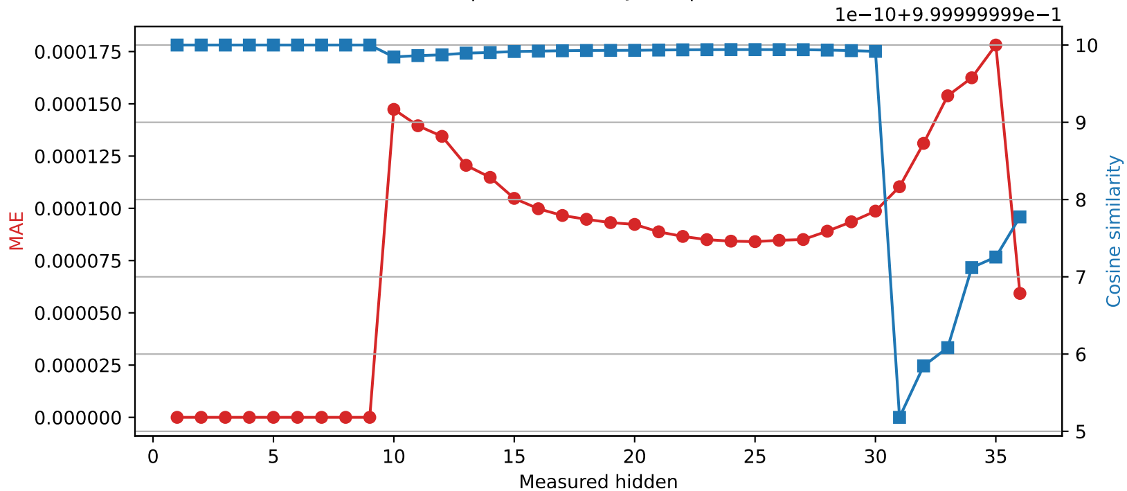
Qwen2.5-3B | Quantized layer 9 | float64 → int16
