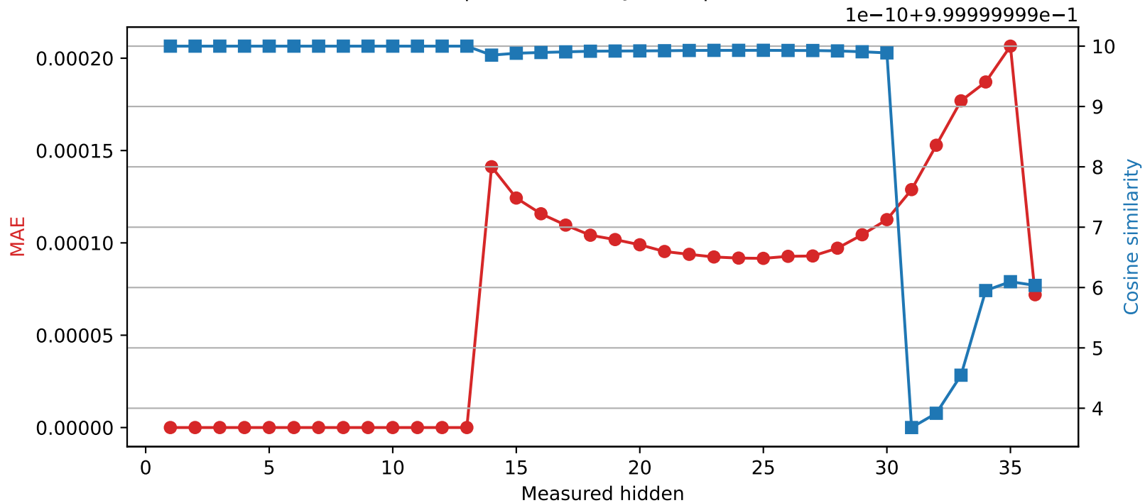
Qwen2.5-3B | Quantized layer 13 | float64 → int16
