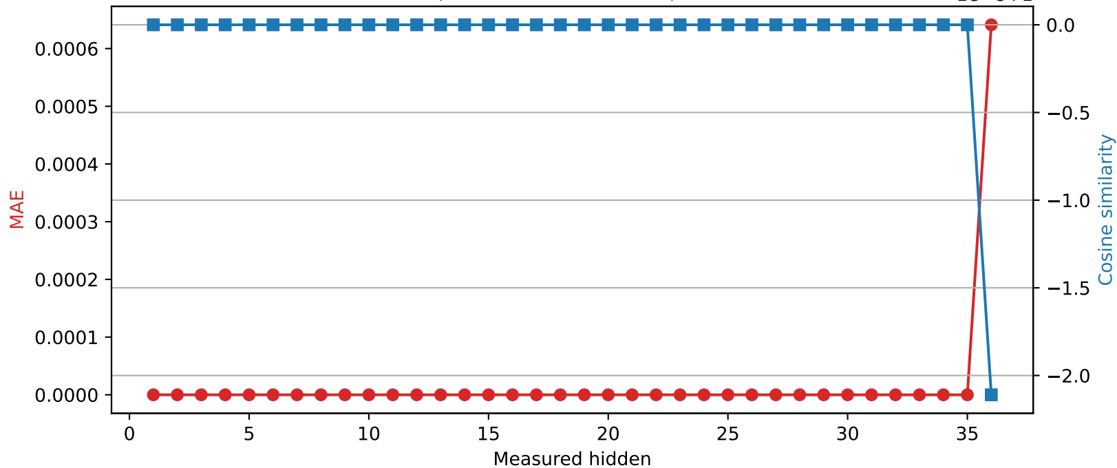
Qwen2.5-3B | Quantized layer 35 | float64 → int16
