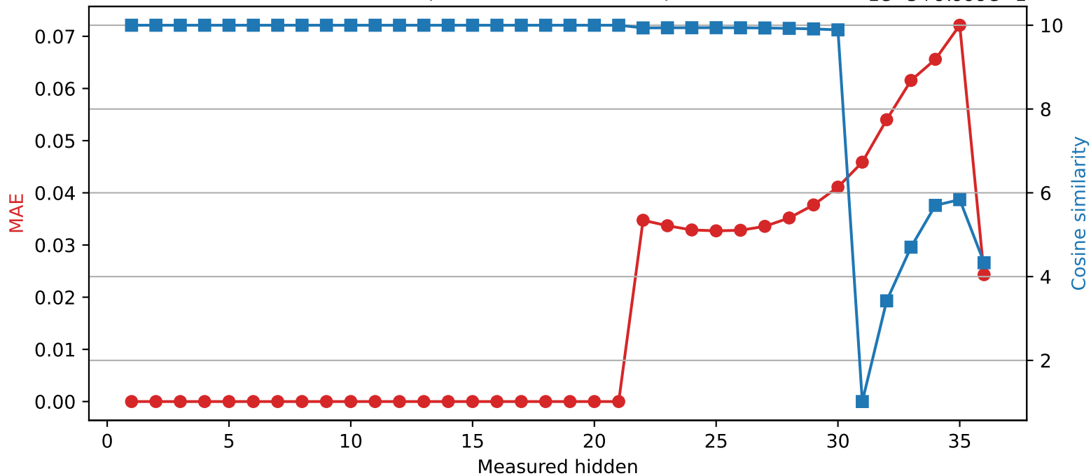
Qwen2.5-3B | Quantized layer 21 | float16 → int8
