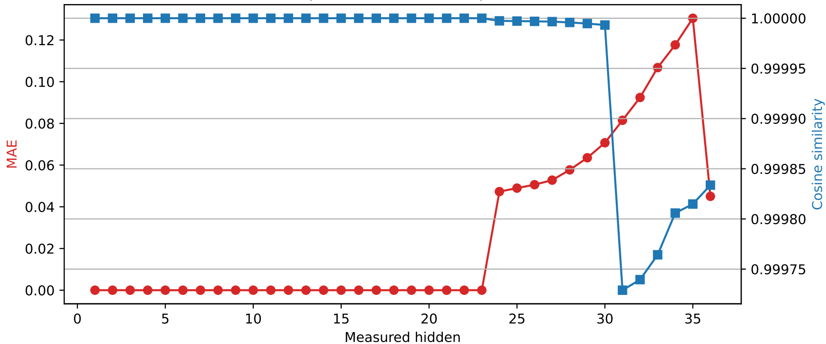
Qwen2.5-3B | Quantized layer 23 | float16 → int8
