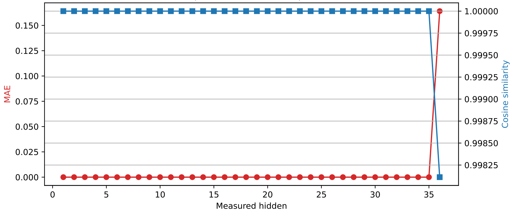
Qwen2.5-3B | Quantized layer 35 | float16 → int8
