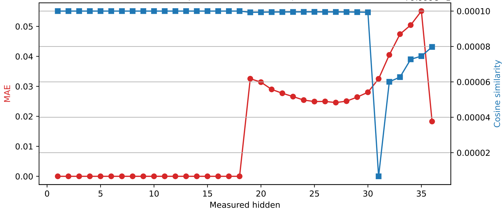
Qwen2.5-3B | Quantized layer 18 | float16 → int8
