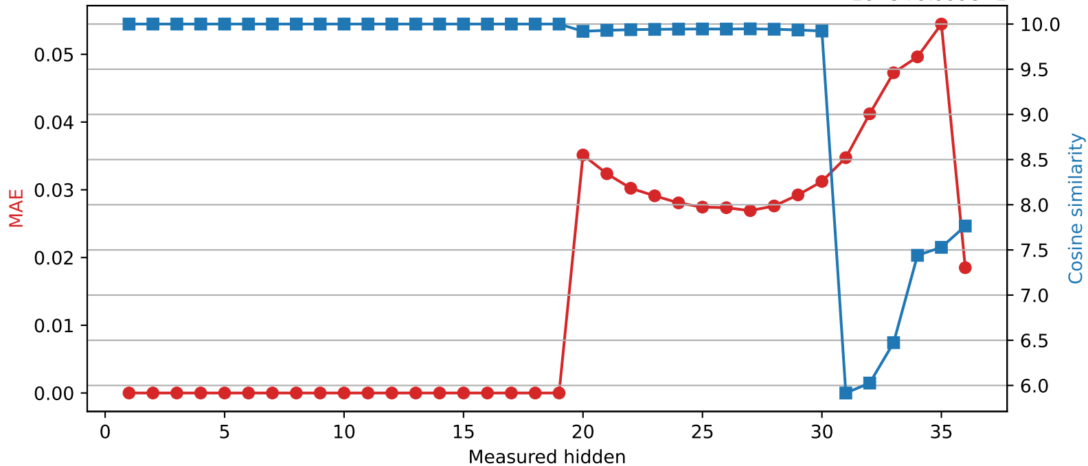
Qwen2.5-3B | Quantized layer 19 | float16 → int8
