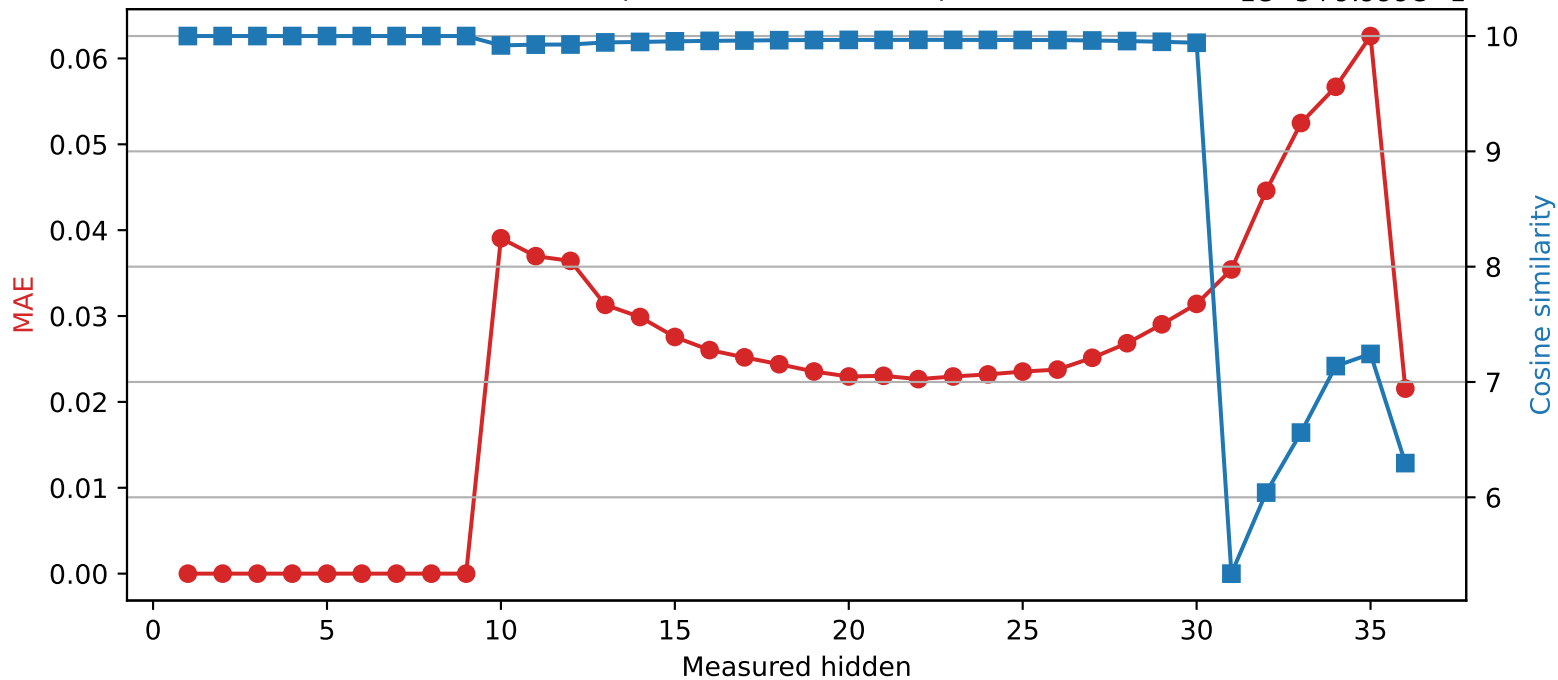
Qwen2.5-3B | Quantized layer 9 | float32 → int8
