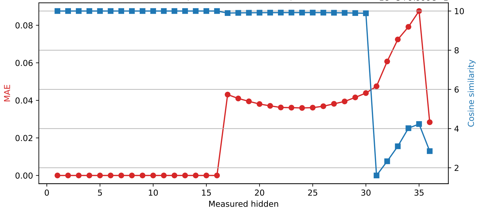
Qwen2.5-3B | Quantized layer 16 | float32 → int8
