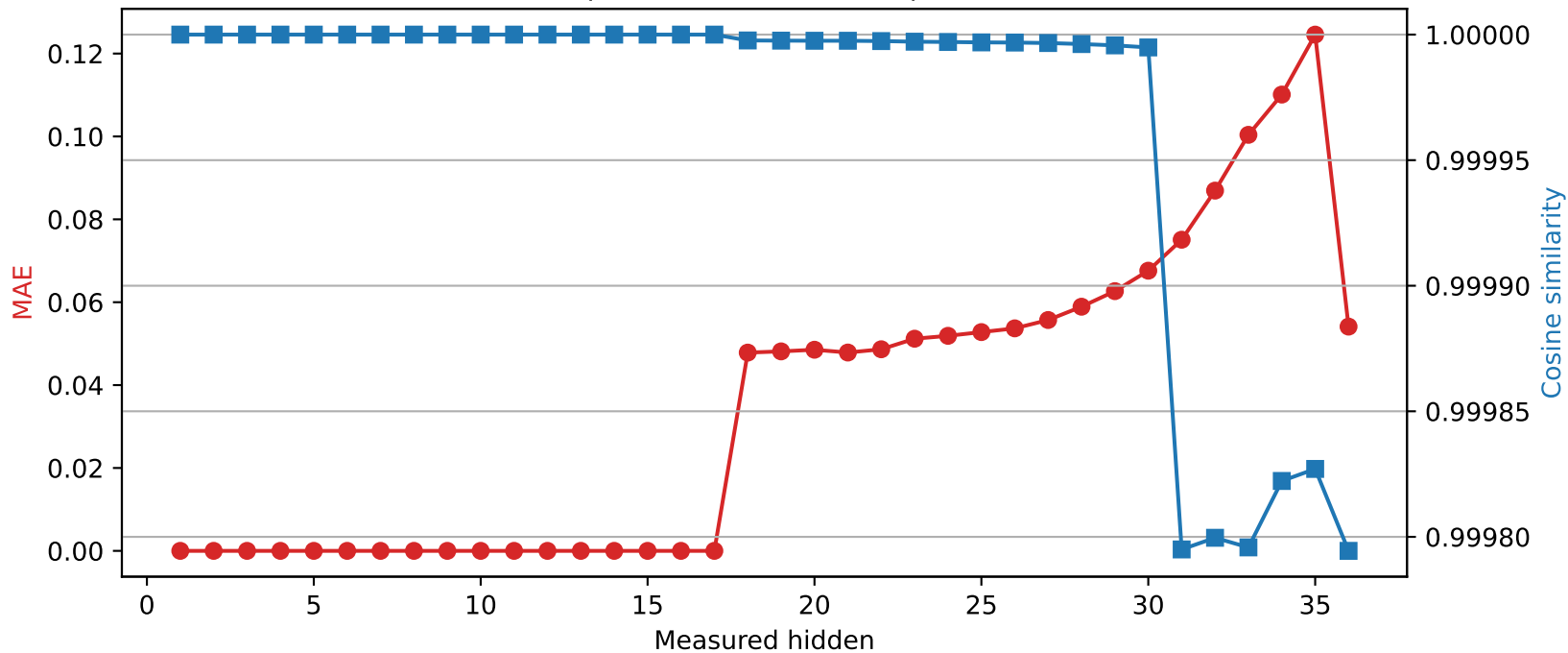
Qwen2.5-3B | Quantized layer 17 | float32 → int8
