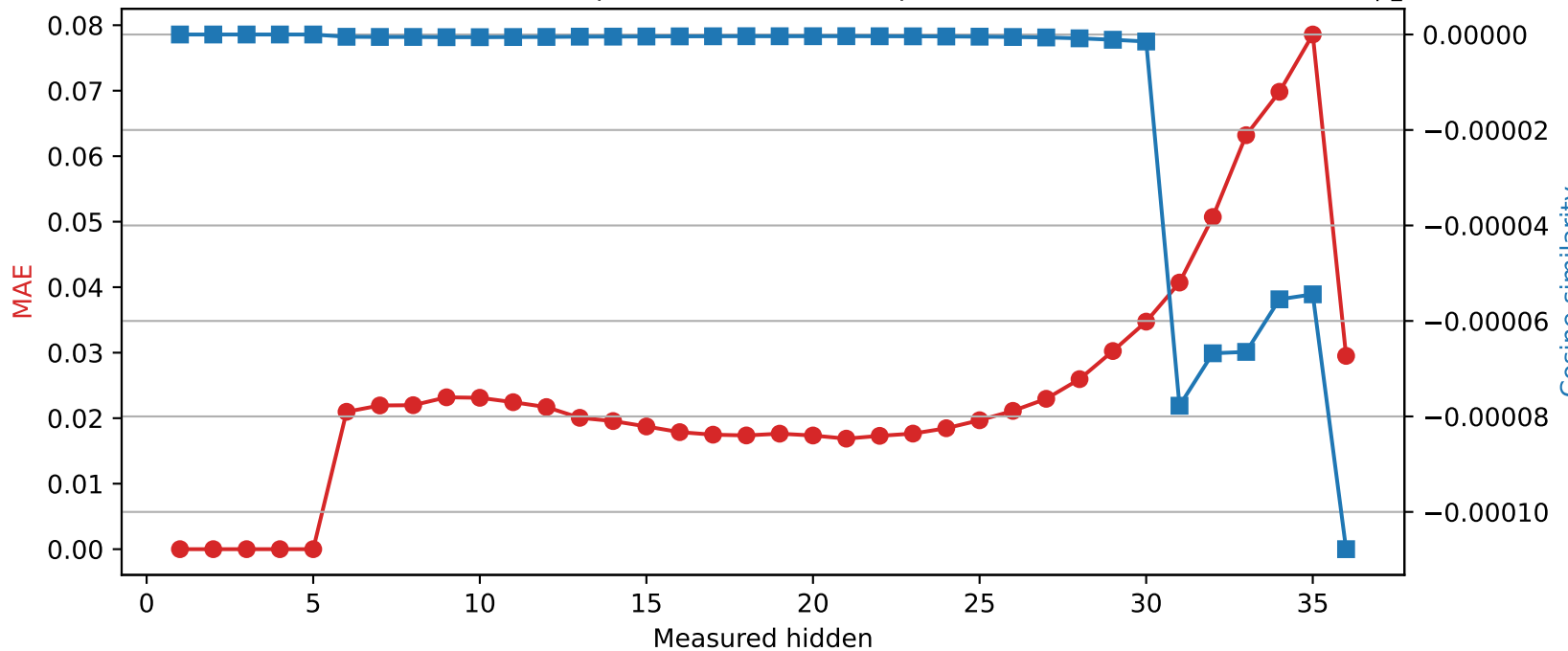
Qwen2.5-3B | Quantized layer 5 | float32 → int8
