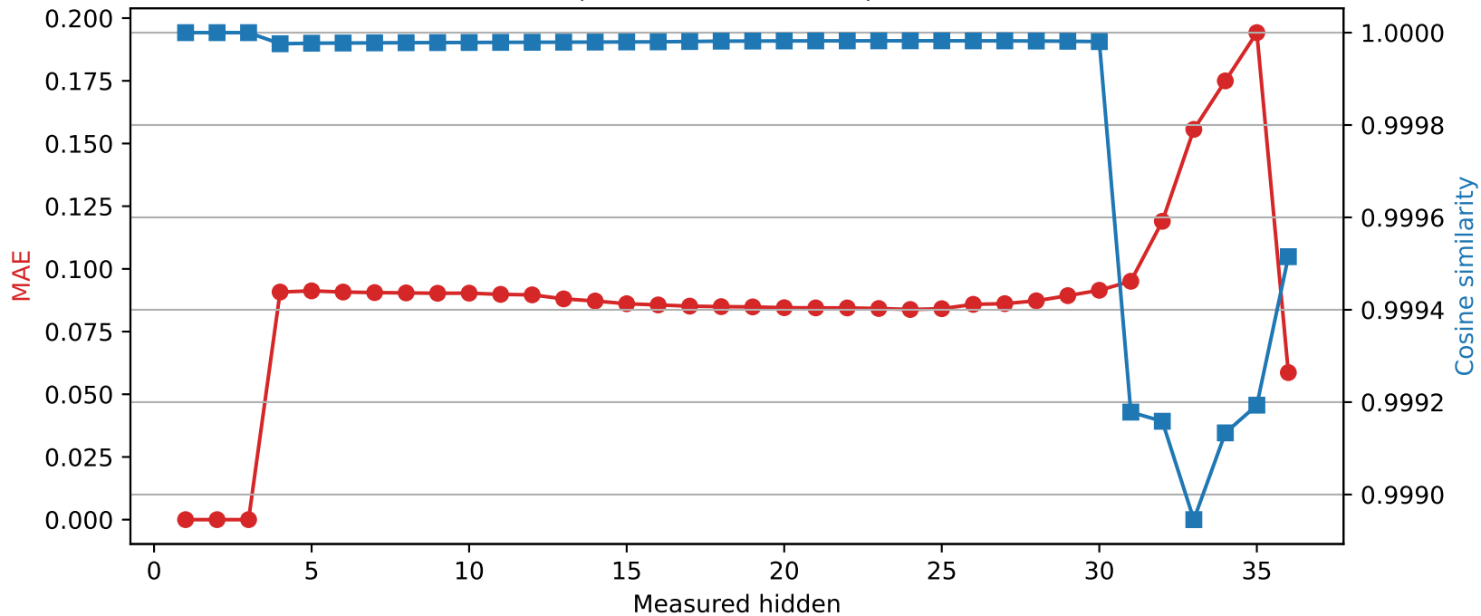
Qwen2.5-3B | Quantized layer 3 | float32 → int8
