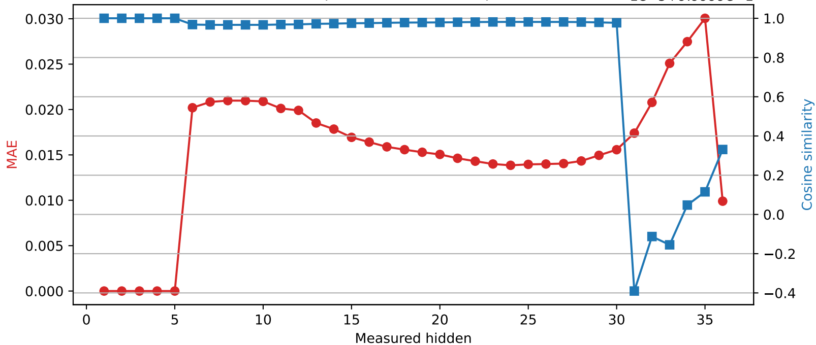
Qwen2.5-3B | Quantized layer 5 | float32 → int8
