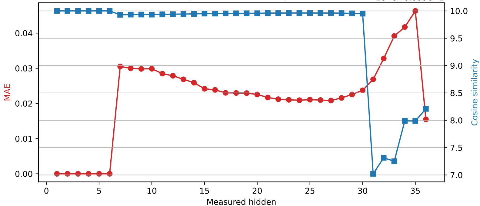
Qwen2.5-3B | Quantized layer 6 | float32 → int8
