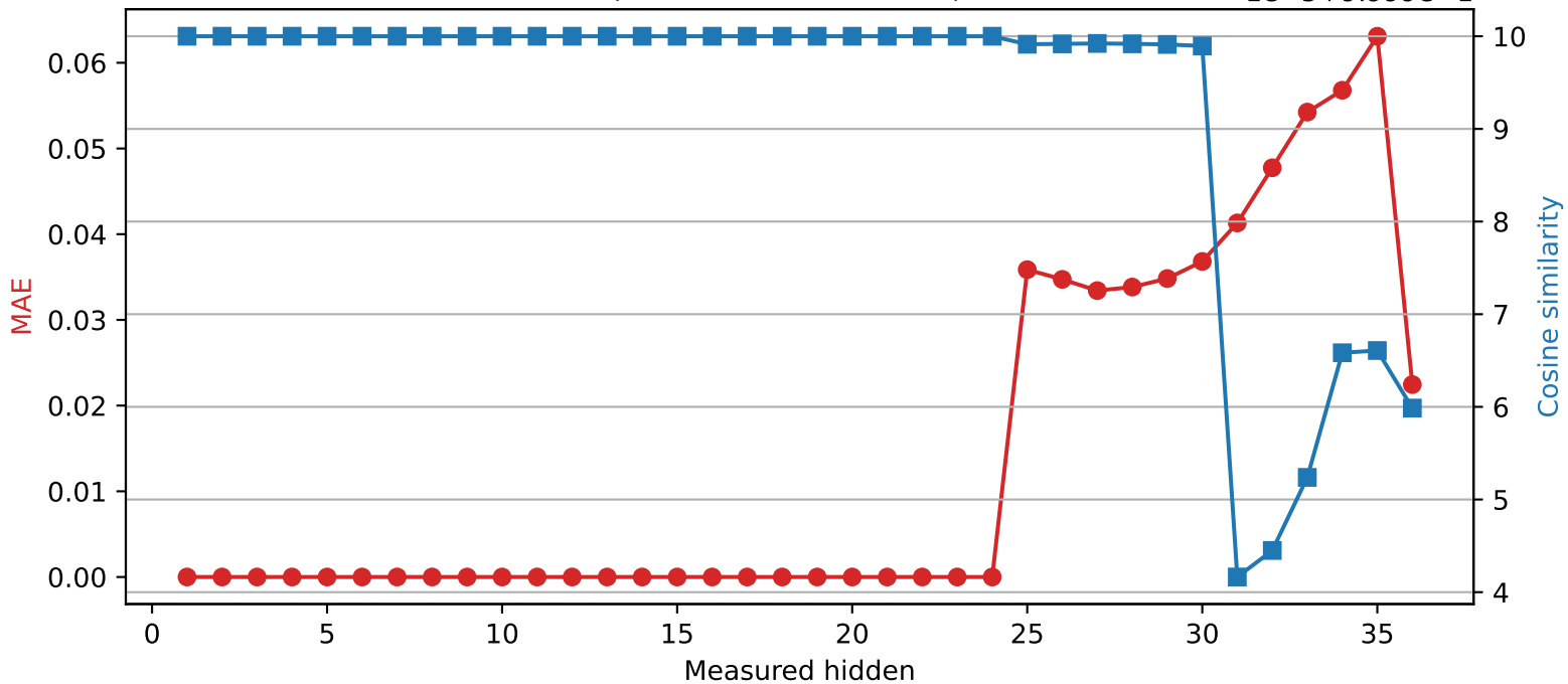
Qwen2.5-3B | Quantized layer 24 | float32 → int8
