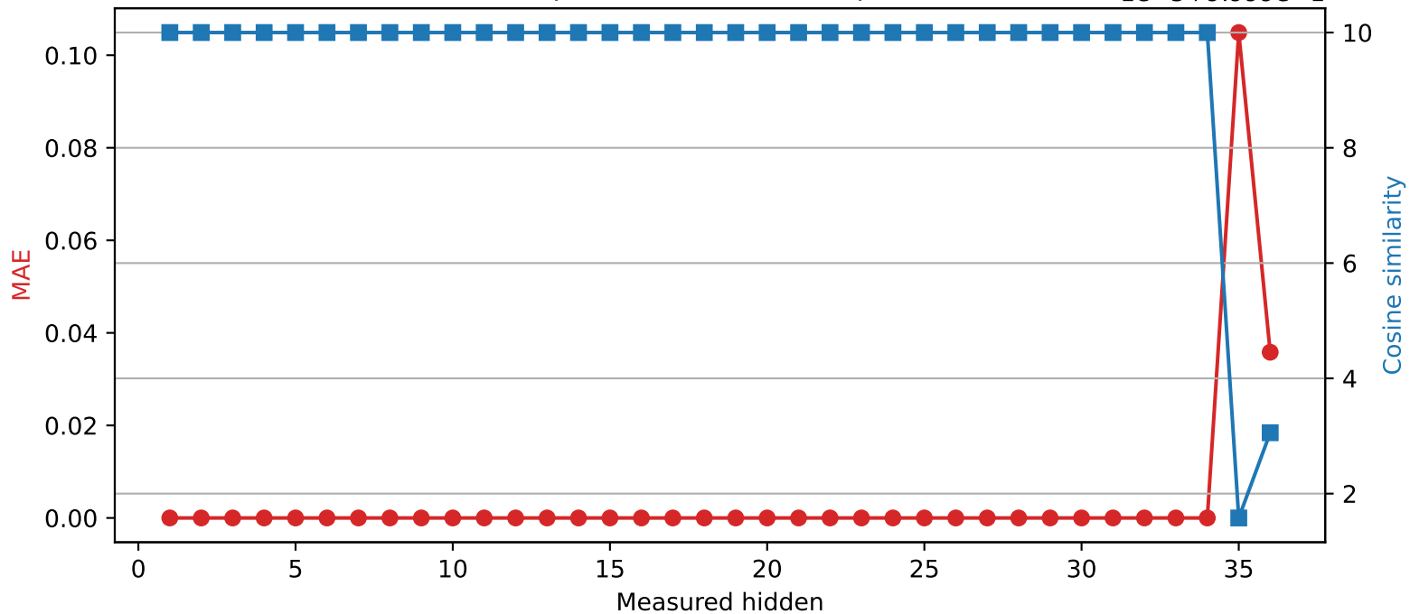
Qwen2.5-3B | Quantized layer 34 | float32 → int8
