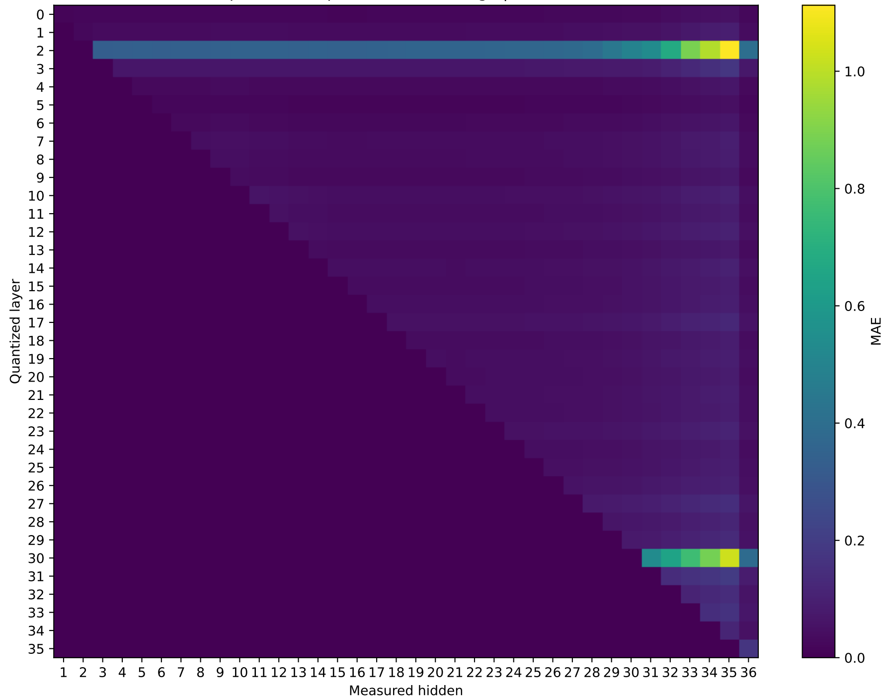
Qwen2.5-3B Prompt 2: MAE representation damage | float64 → int8
