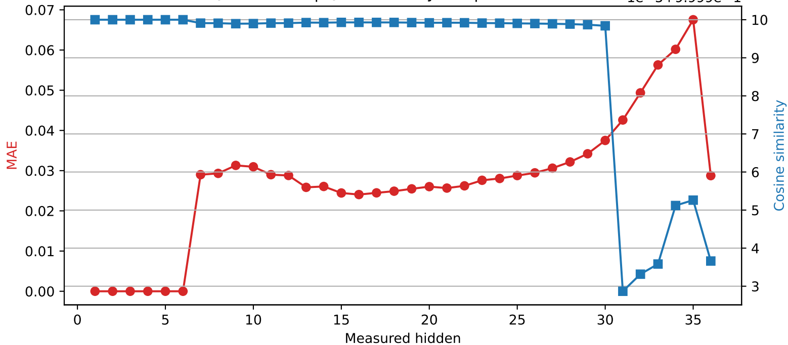
Qwen2.5-3B | Quantized layer 6 | float64 → int8
