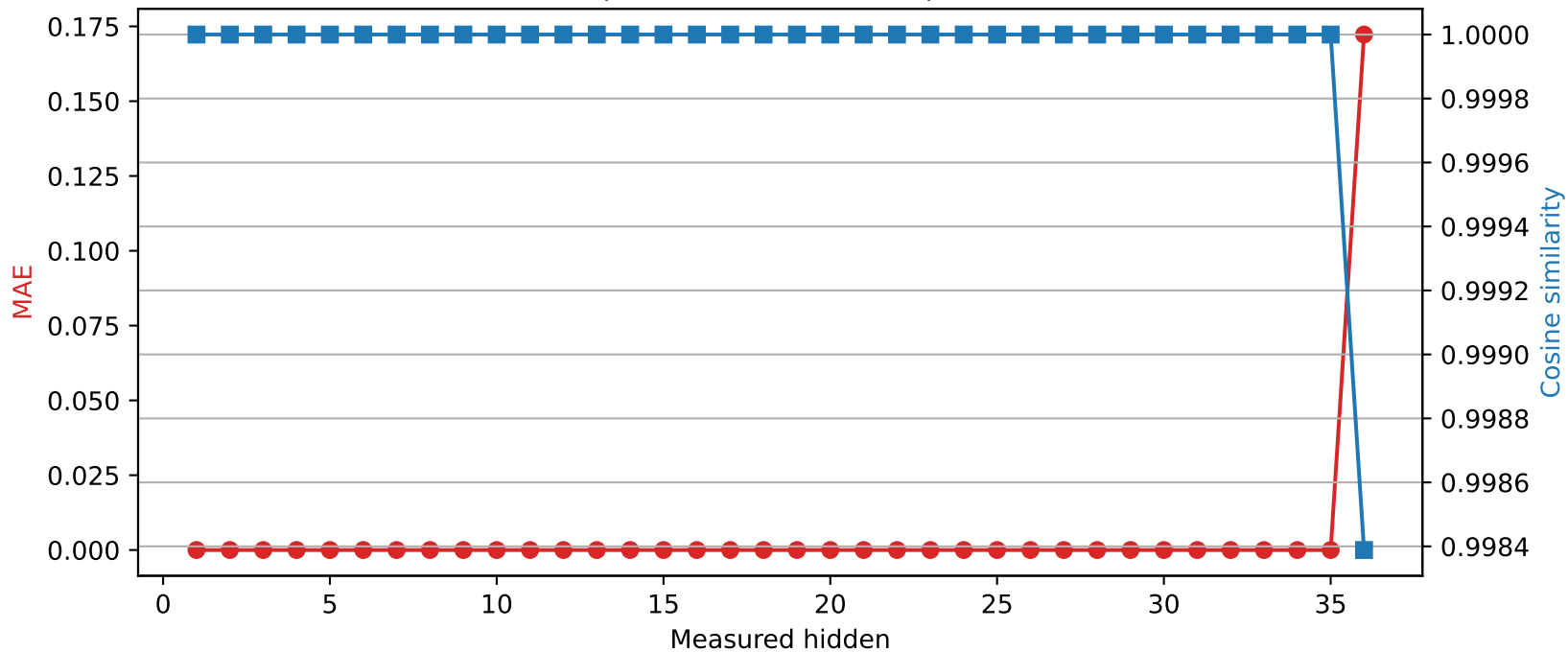
Qwen2.5-3B | Quantized layer 35 | float64 → int8
