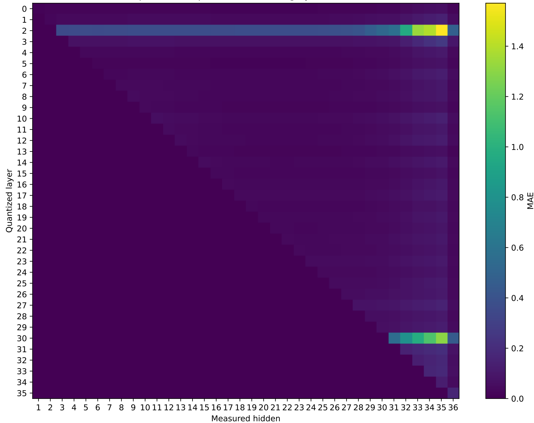
Qwen2.5-3B Prompt 3: MAE representation damage | float64 → int8
