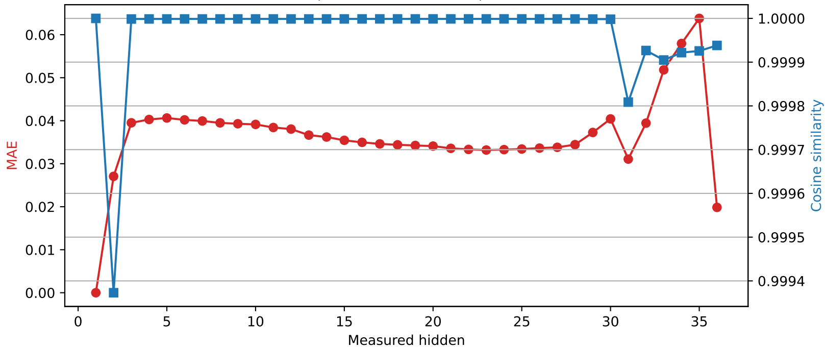
Qwen2.5-3B | Quantized layer 1 | float64 → int8
