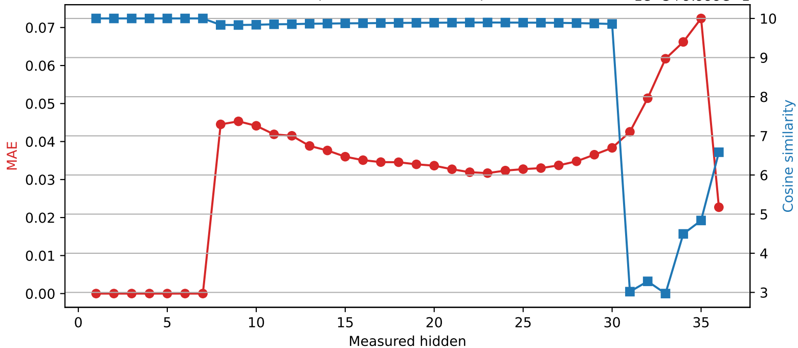
Qwen2.5-3B | Quantized layer 7 | float64 → int8
