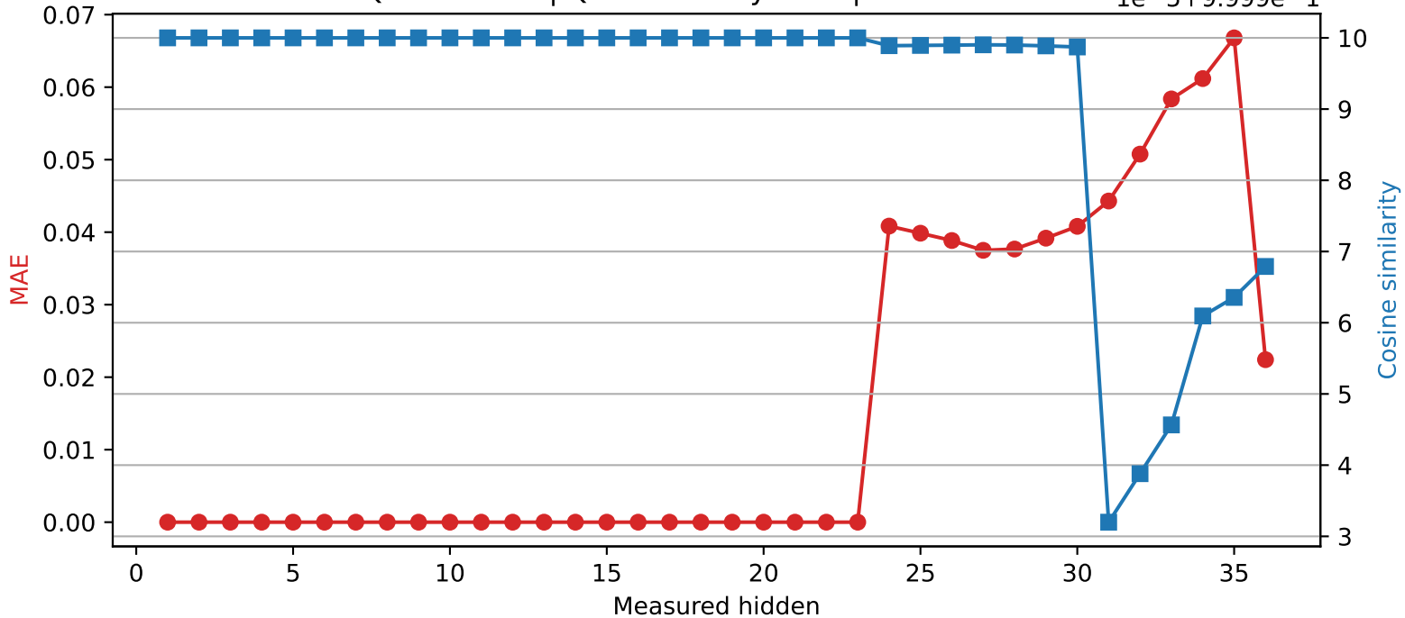
Qwen2.5-3B | Quantized layer 23 | float64 → int8
