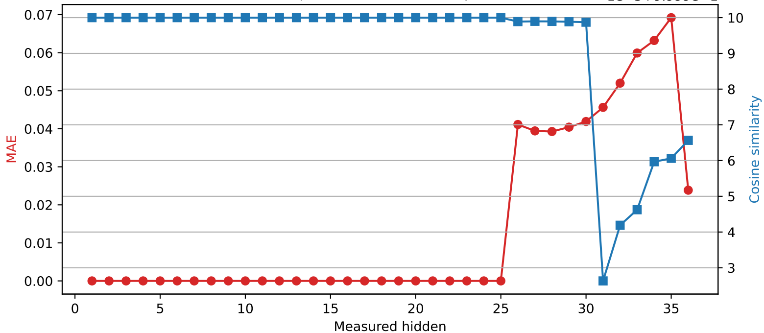
Qwen2.5-3B | Quantized layer 25 | float64 → int8
