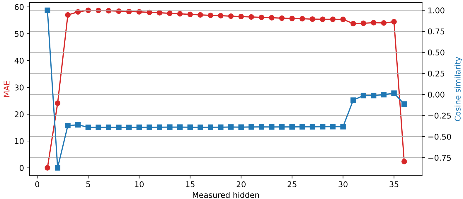
Qwen2.5-3B | Quantized layer 1 | float16 → int4
