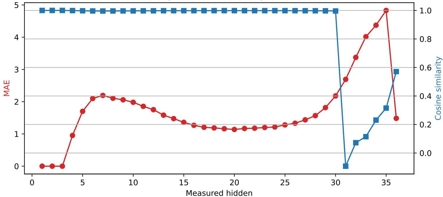
Qwen2.5-3B | Quantized layer 3 | float16 → int4
