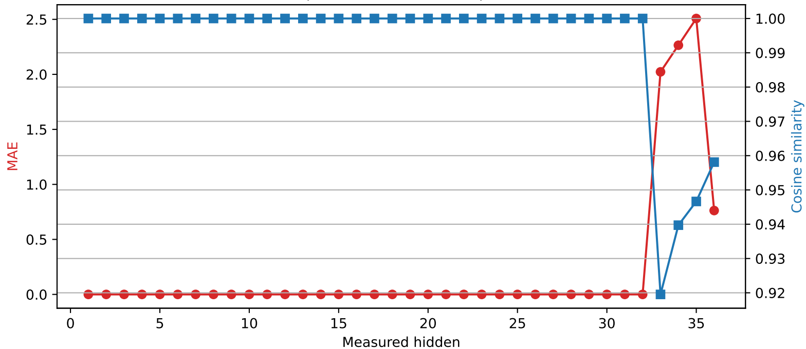
Qwen2.5-3B | Quantized layer 32 | float16 → int4
