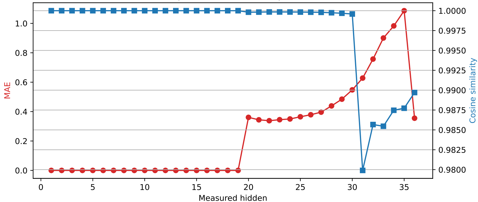
Qwen2.5-3B | Quantized layer 19 | float16 → int4
