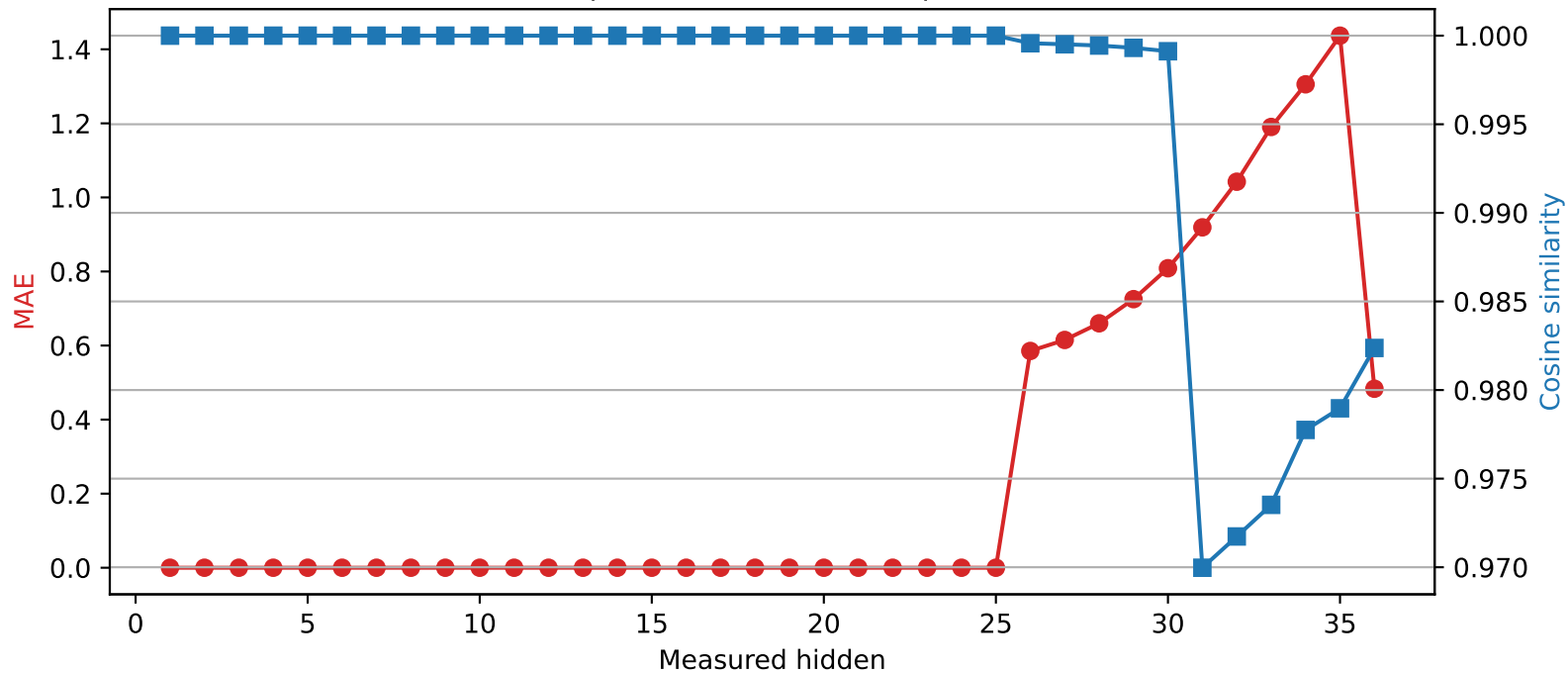
Qwen2.5-3B | Quantized layer 25 | float16 → int4
