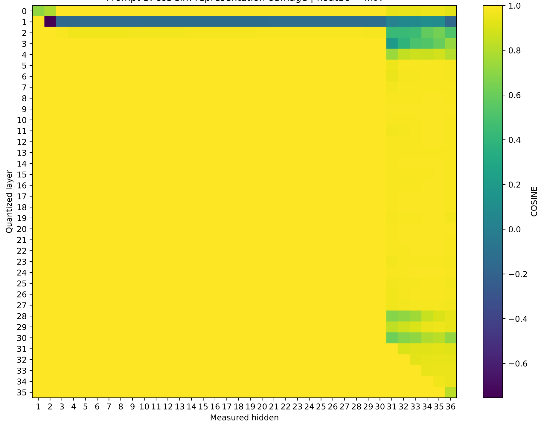
Qwen2.5-3B Prompt 3: cos sim representation damage | float16 → int4
