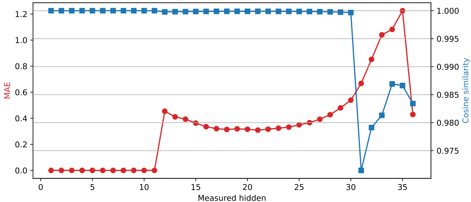
Qwen2.5-3B | Quantized layer 11 | float16 → int4
